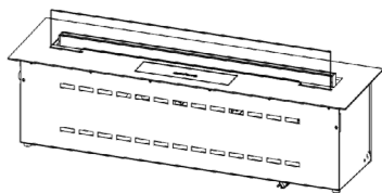
GLASS SOLUTION 1 1 glass in front of burner. Hight: 65mm Thickness: 4mm
