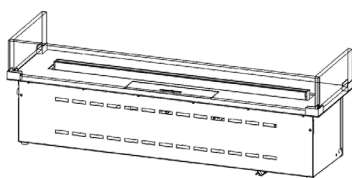
GLASS SOLUTION 7 3 glasses on top plate edge. Hight: 80mm Thickness: 10mm
