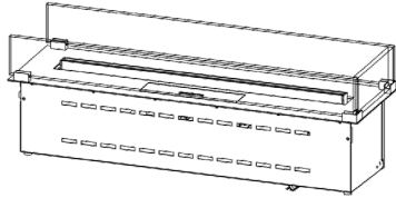
GLASS SOLUTION 5 3 glasses on top plate edge. Hight: 80mm Thickness: 10mm
