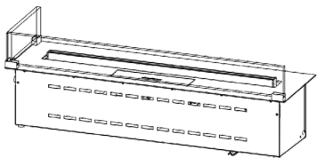
GLASS SOLUTION 8 2 glasses on top plate edge. Hight: 80mm Thickness: 10mm
