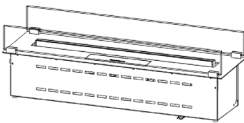
GLASS SOLUTION 4 2 glasses on top plate edge. Hight: 80mm Thickness: 10mm
