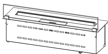
GLASS SOLUTION 3 1 glasses on top plate edge. Hight: 80mm Thickness: 10mm
