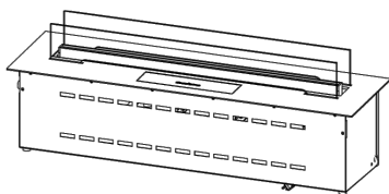
GLASS SOLUTION 2 2 glasses in front of burner. Hight: 65mm Thickness: 4mm
