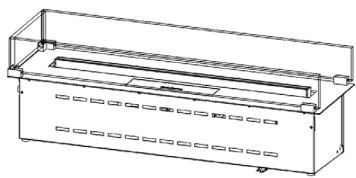
GLASS SOLUTION 6 3 glasses on top plate edge. Hight: 80mm Thickness: 10mm
